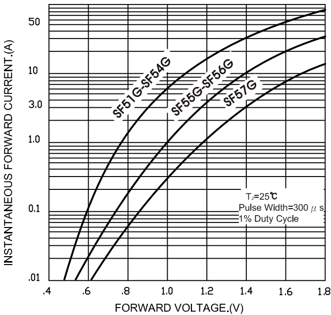
FIG.3-TYPICAL FORWARD CHARACTERISTICS
