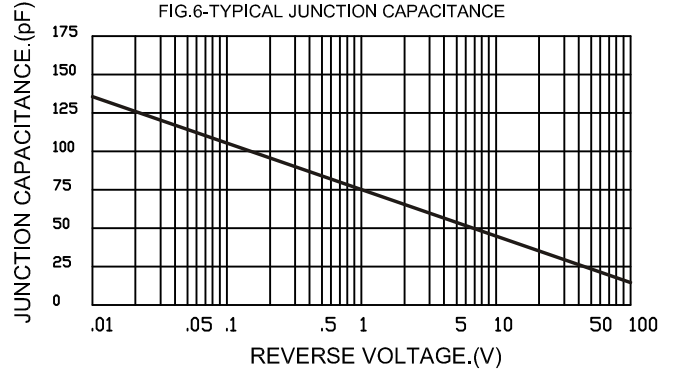
FIG.6-TYPICAL JUNCTION CAPACITANCE
