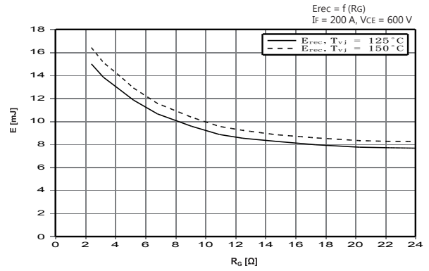
Fig.10 Switching losses Diode, Inverter (typical)
