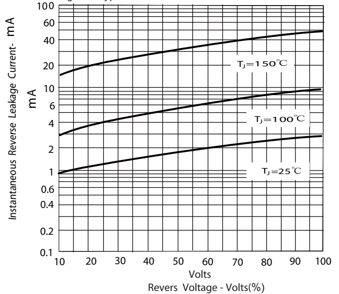
Figure.4-Typical Reverse Characteristics
